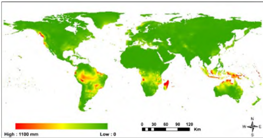
Fig. 2. Global Precipitation map of January 1973 obtained from CruTS 3.23 data.
