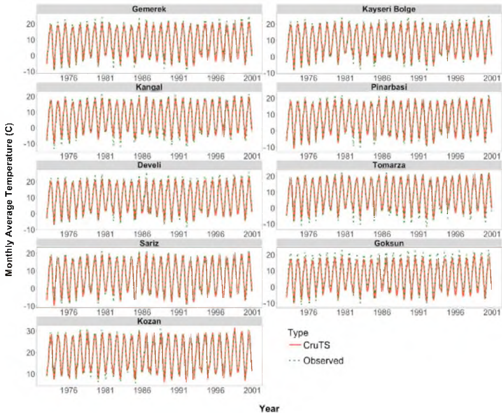
Fig. 6. Time series plot of the monthly average temperature obtained from CruTS and Observed data for the period 1973 - 2000.
