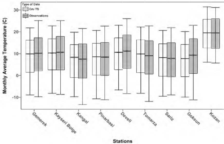
Fig. 4. CruTS and observed temperature data boxplot.
