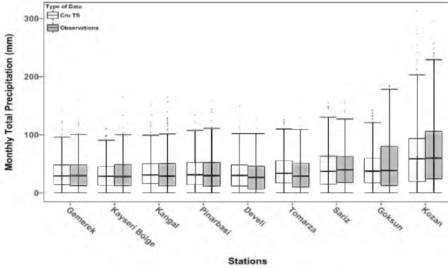
Fig. 3. CruTS and observed precipitation data boxplot.
