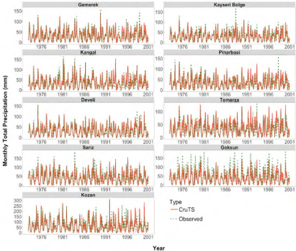
Fig. 5. Time series plot of the monthly total precipitation obtained from CruTS and Observed data for the period 1973 - 2000.
