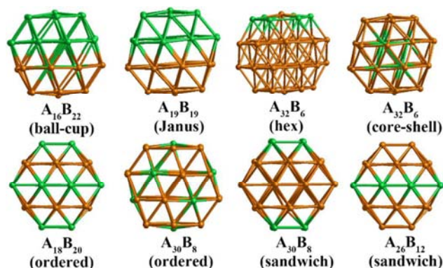
Figure 2. Examples of 38-TO nanoalloys with different compositions and chemical arrangements. The "hex" configuration has the central atom of one (111) facet surrounded by a hexagon of six atoms of the other element.
