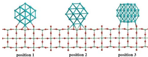
Figure 3. The three positions studied for 38-TO Pd-Ir and Au-Rh nanoalloy clusters (and their pure metal equivalents) adsorbed on the TiO 2 (110) surface.
