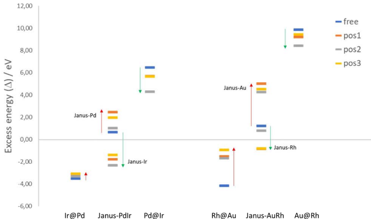
Figure 6. Excess energies of free and \text{TiO}_2 -supported Pd-Ir and Au-Rh 38-TO clusters with core-shell (A@B) and Janus configurations. The coloured bars represent the free NP and the three different binding positions on the support.
