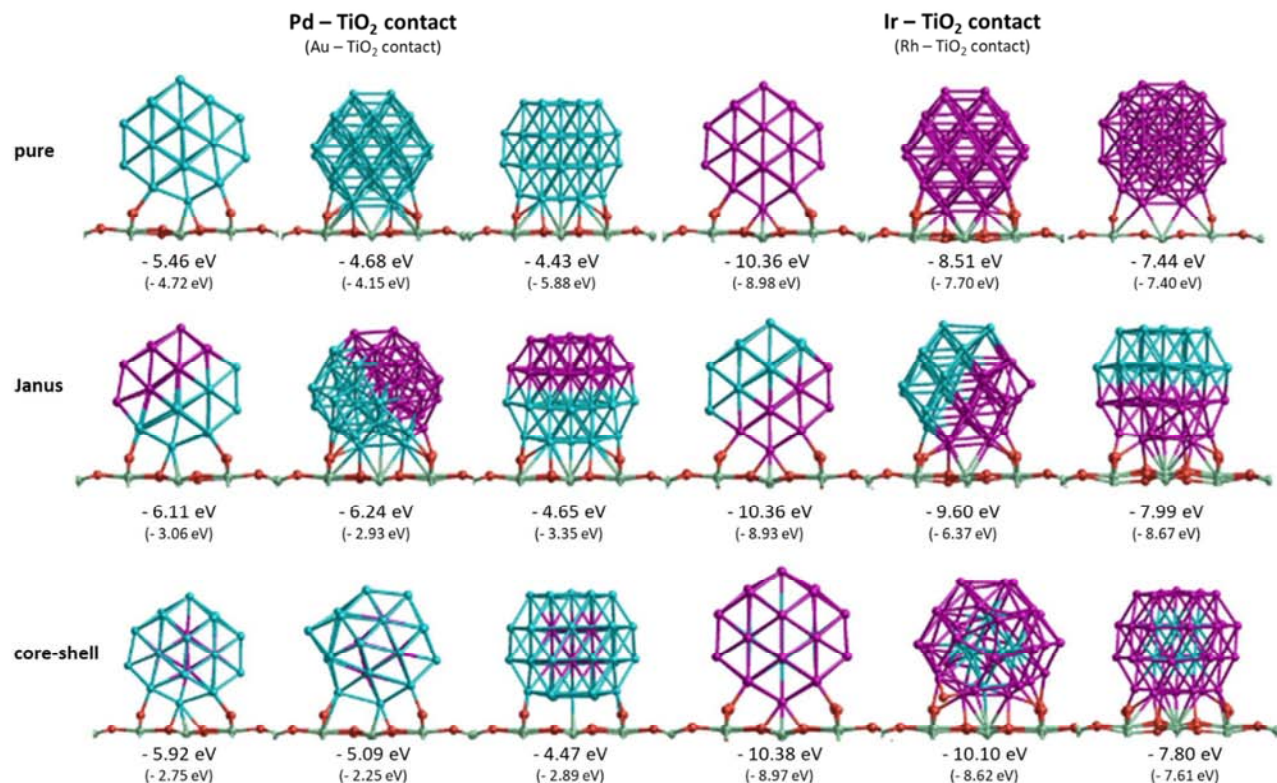
Figure 5. Structures and corresponding surface binding energies ( E_{s\text{-bind}} ) for 38-atom pure Pd and Ir clusters and Pd-Ir nanoalloys supported on \text{TiO}_2(110) in three orientations. The surface binding energies of Au-Rh clusters, corresponding to the same structures (with Au replacing Pd and Rh replacing Ir), are given in parentheses. Pd, Ir, O and Ti atoms are represented in blue, purple, red and green, respectively. For simplicity, only the top layer of the \text{TiO}_2 slab is shown.
