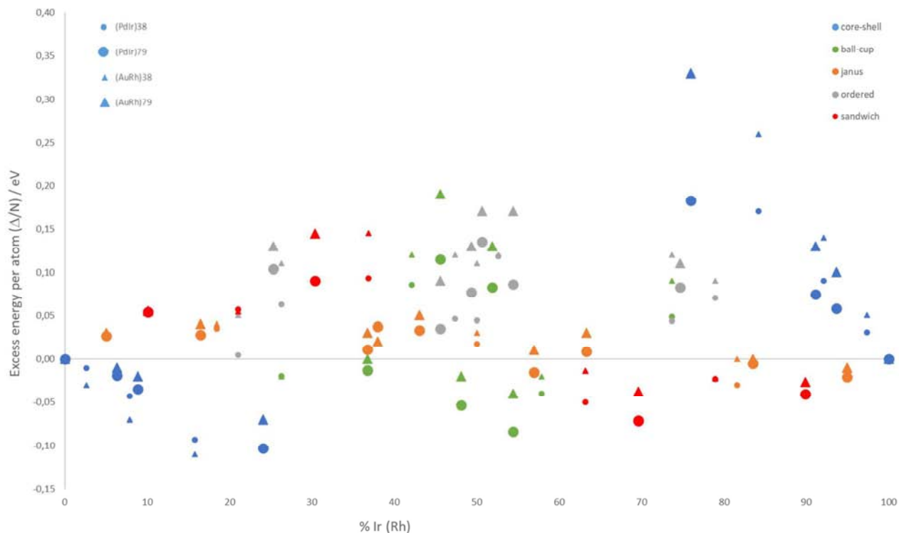
Figure 4. Excess energy per atom ( \Delta/N ) versus atomic composition for 38-TO and 79-TO Pd-Ir and Au-Rh nanoalloys.
