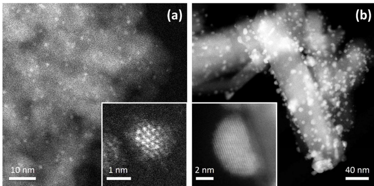
Figure 1. Experimental HAADF-STEM images of supported Pd-Ir and Au-Rh nanoparticles. (a) Image of 2 \pm 1 nm Pd-Ir nanoparticles supported on \gamma - \text{Al}_2\text{O}_3 . The catalyst was prepared by incipient wetness co-impregnation of the support with Pd and Ir acetylacetonates followed by thermal treatment in \text{H}_2 . 7 The insert shows a high-resolution image of a single particle: the Z-contrast indicates a core-shell structure, consistent with an Ir-rich core and a Pd-rich shell. (b) Image of 4 \pm 1 nm Au-Rh nanoparticles supported on rutile \text{TiO}_2 nanorods. The sample was prepared by chemical co-reduction and sol immobilization, followed by treatment in \text{H}_2 at 350^\circ\text{C} . 18,22 The insert shows a high-resolution image of a single particle: the Z-contrast indicates a faceted Janus particle, with Rh at the interface between Au and the \text{TiO}_2 substrate.
