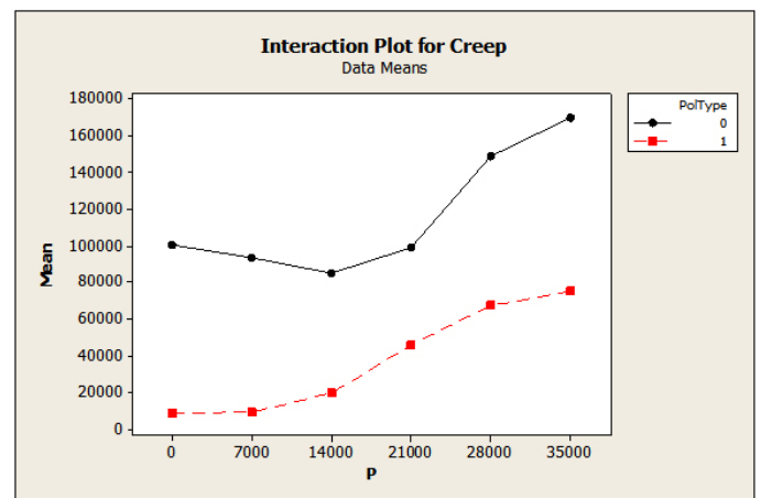
Fig. 11. Interaction plot for polypropylene type versus pulse counts
