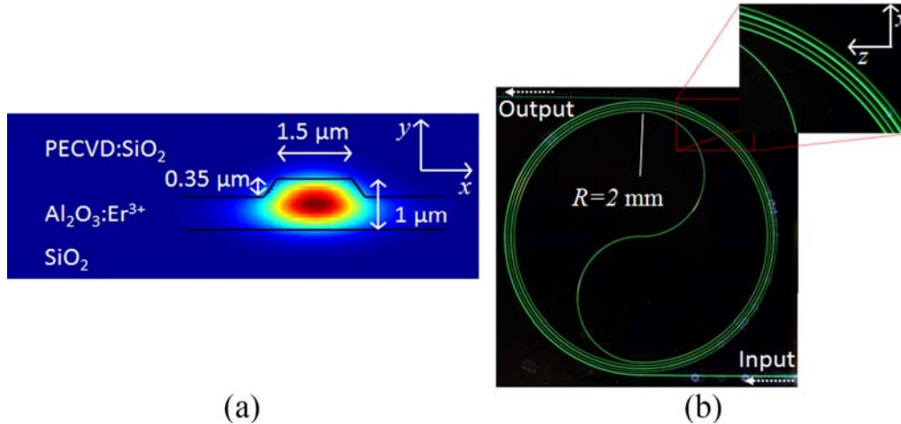
Fig. 1. (a) Waveguide amplifier cross-section and simulated signal-mode profile. (b) Photograph of a pumped ( \lambda_p = 976 nm) \text{Al}_2\text{O}_3:\text{Er}^{3+} spiral amplifier on a silicon chip. A close-up view of the spiral amplifier is shown in the inset.
