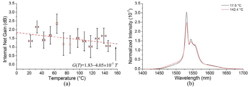
Fig. 6. (a) Measured internal net gain at different sample temperatures for the 12.9-cm-long spiral waveguide with an \text{Er}^{3+} concentration of 0.95 \times 10^{20} \text{ cm}^{-3} . A linear fit is shown as a dashed line. (b) Normalized amplified-spontaneous-emission spectra recorded at 17.5 and 142.4°C.
