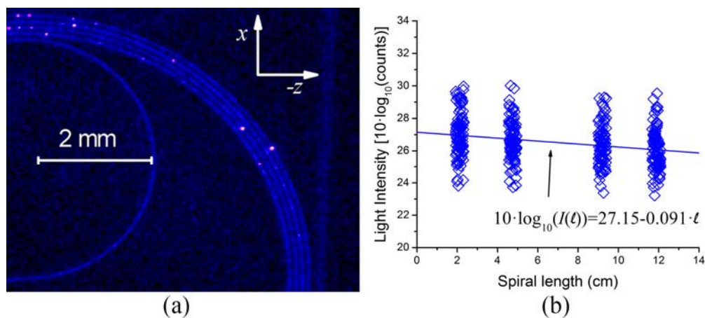
Fig. 2. (a) Infrared image ( \lambda = 1320 nm) of a quarter of a spiral-shaped channel waveguide. (b) Intensity distribution along the propagation direction in the spiral-shaped channel waveguide measured by applying the imaging method described in [28].
