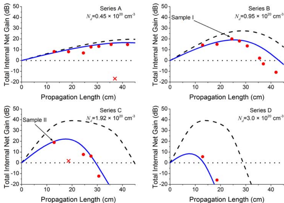
Fig. 3. Internal net gain in \text{Al}_2\text{O}_3:\text{Er}^{3+} spiral waveguide amplifiers: simulations with (solid blue curves) and without (dashed black curves) considering the fraction of quenched ions, and measurements (red circles) for different waveguide lengths and \text{Er}^{3+} concentrations of 0.45 \times 10^{20} \text{ cm}^{-3} (Series A), 0.95 \times 10^{20} \text{ cm}^{-3} (Series B), 1.92 \times 10^{20} \text{ cm}^{-3} (Series C), and 3.0 \times 10^{20} \text{ cm}^{-3} (Series D). Simulations are based on the quenched-ion amplifier model [13] and the parameters given in Table 1.
