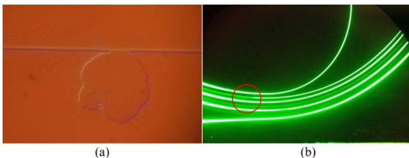
Fig. 4. (a) Defect in contact with the waveguide. (b) Drop of green upconversion luminescence as a result of pump power scattered at the defect location (red circle).
