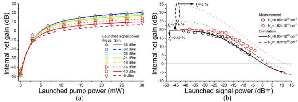
Fig. 5. (a) Measured (symbols) and simulated (curves) internal net gain at different launched signal powers for the 12.9-cm-long spiral waveguide with an \text{Er}^{3+} concentration of 1.92 \times 10^{20} \text{ cm}^{-3} at different pump powers. (b) Maximum internal net gain as a function of launched signal power for two samples with concentrations of 0.95 \times 10^{20} \text{ cm}^{-3} (black) and 1.92 \times 10^{20} \text{ cm}^{-3} (red) and lengths of 24.45 and 12.91 cm, respectively. The data points show the measured values, while the continuous, dashed, and dotted curves show the simulated values including and excluding f_c , respectively.
