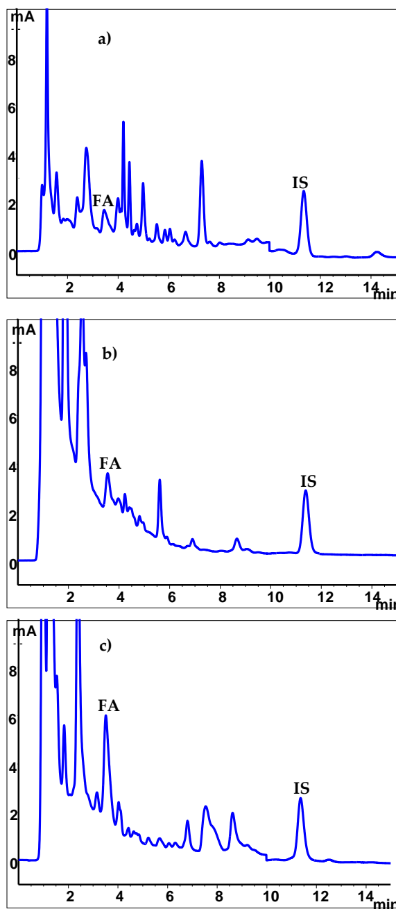
Figure 2. Representative chromatograms obtained from malt-based beverages using the proposed UHPLC method a) Boza, b) Vitamin Fortified Malt Beverage, and c) Malt beer sample.
