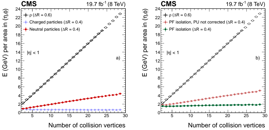
Figure 20. Average energy density as a function of the number of reconstructed proton-proton collision vertices, for electron candidates with p_T > 20\text{GeV} and |\eta| < 1 from data dominated by Z \rightarrow e^+e^- events. The energy density \rho (open dots) is shown, along with each component of the particle isolation: a) neutral particles (red dots) and charged particles associated with the vertex (blue dots), and b) before (pink dots) and after (green dots) the correction for pileup on PF isolation.
