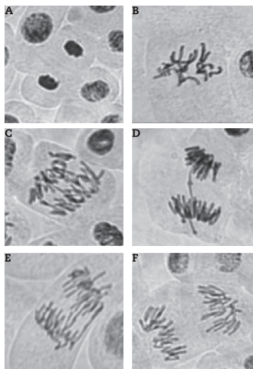
Figure 1 - Some chromosome aberrations of Allium cepa treated with root, stem and leaf extracts of L. globuliferum . A, Sticky chromosomes; B, C-mitosis; C, Three bridges; D, Anaphase bridge; E, Two bridges; F, Laggard chromosomes.
