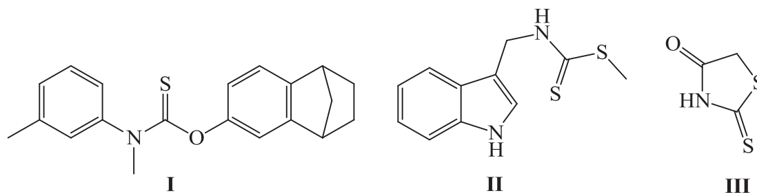
Figure. The chemical structures of the tolclolate (I), brassinin (II), and rhodanine (III).
