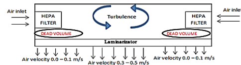
Figure 2. OR Air-ceiling unit with vertical HEPA filter
