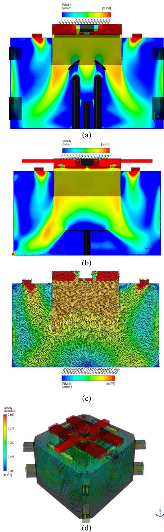
Figure 7. Optimized air velocity distribution for OR, (a) 2D xy coordinates (b) 2D zy coordinates (c) velocity vectors and (d) 3D air velocity distribution
